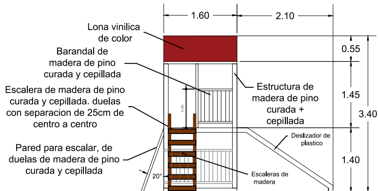
LATERAL SINGLE TOWER
