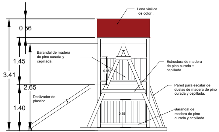
DETALLE DE SINGLE TOWER
