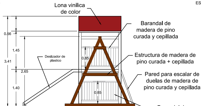
LATERAL SINGLE TOWER
