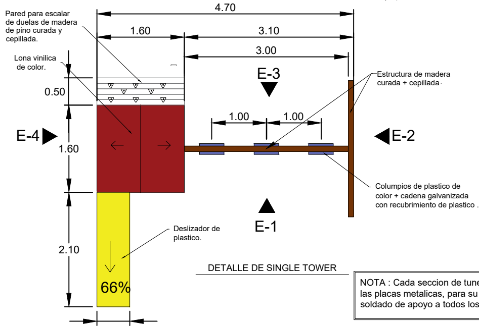
DETALLE DE SINGLE TOWER
