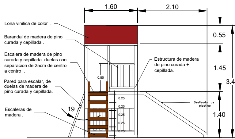
DETALLE DE SINGLE TOWER
