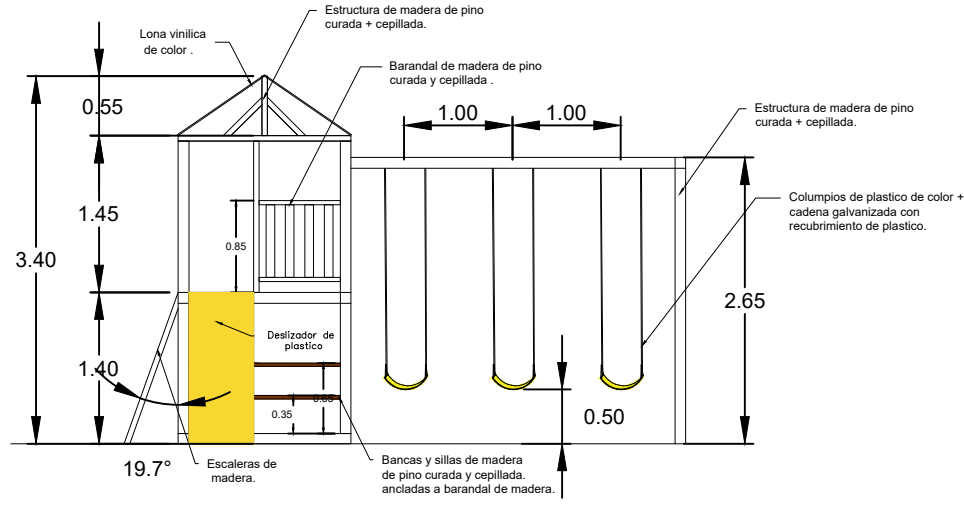
DETALLE DE SINGLE TOWER
