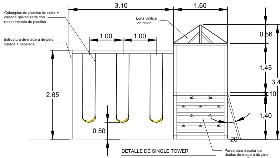
DETALLE DE SINGLE TOWER
